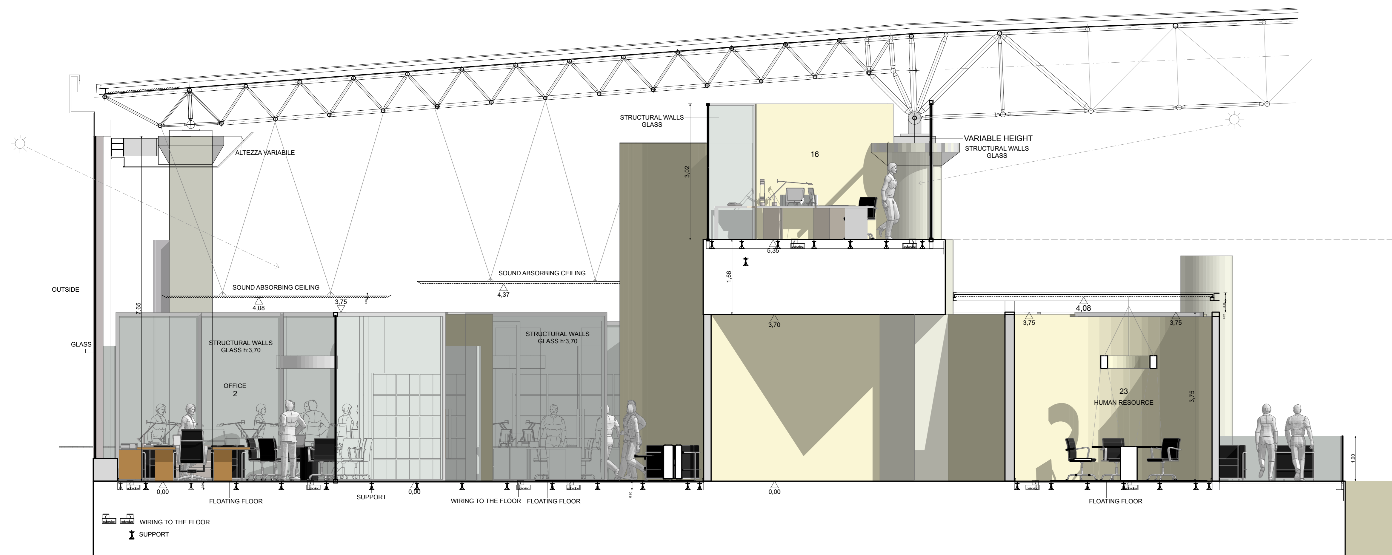
SECTION ELEVATION A-05
