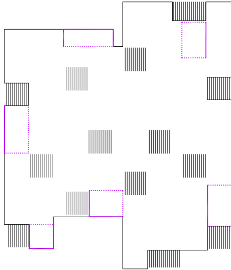
voids and volumes
