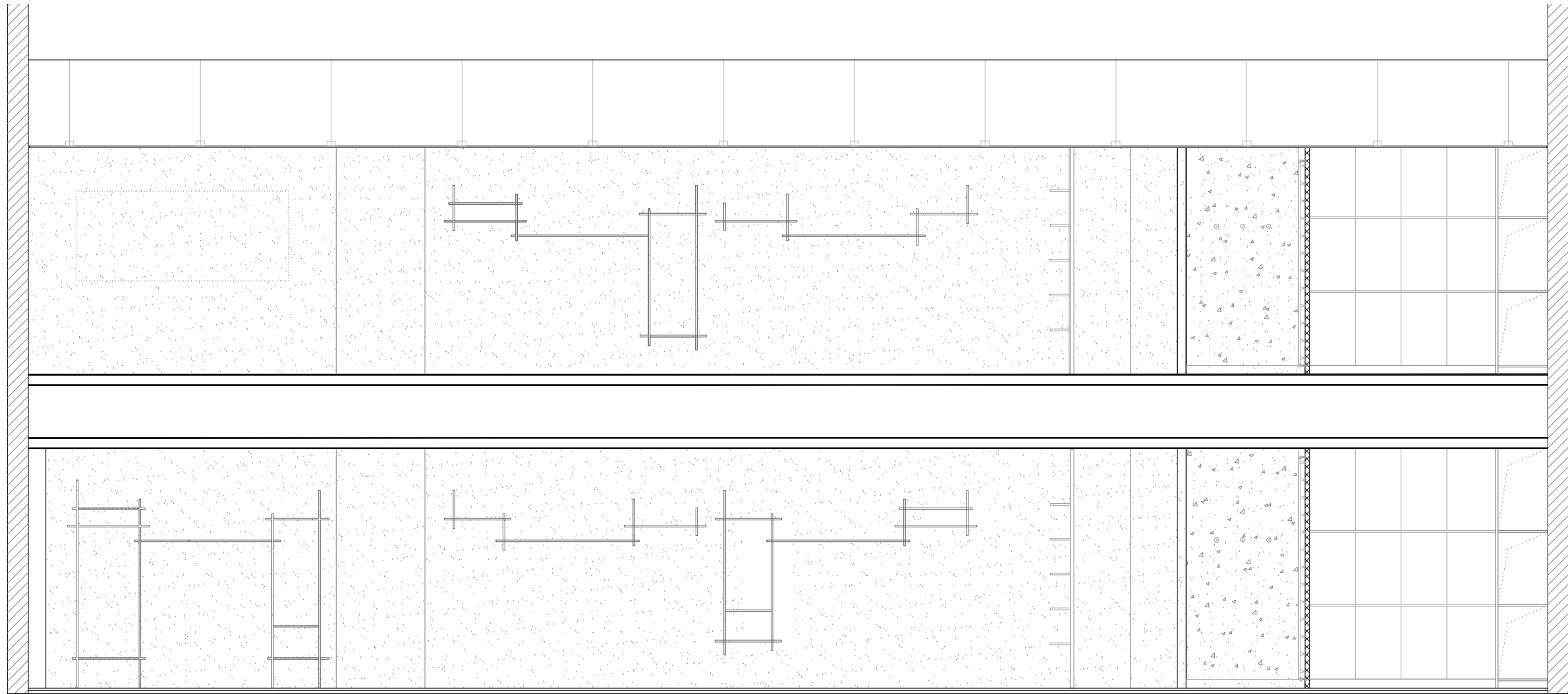
Interior Elevation
