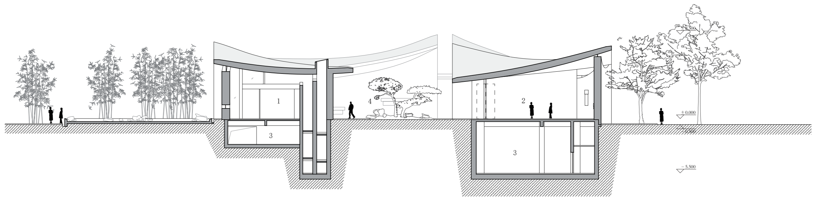
Section 1-1
