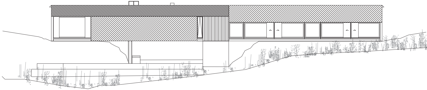
Northwest elevation
