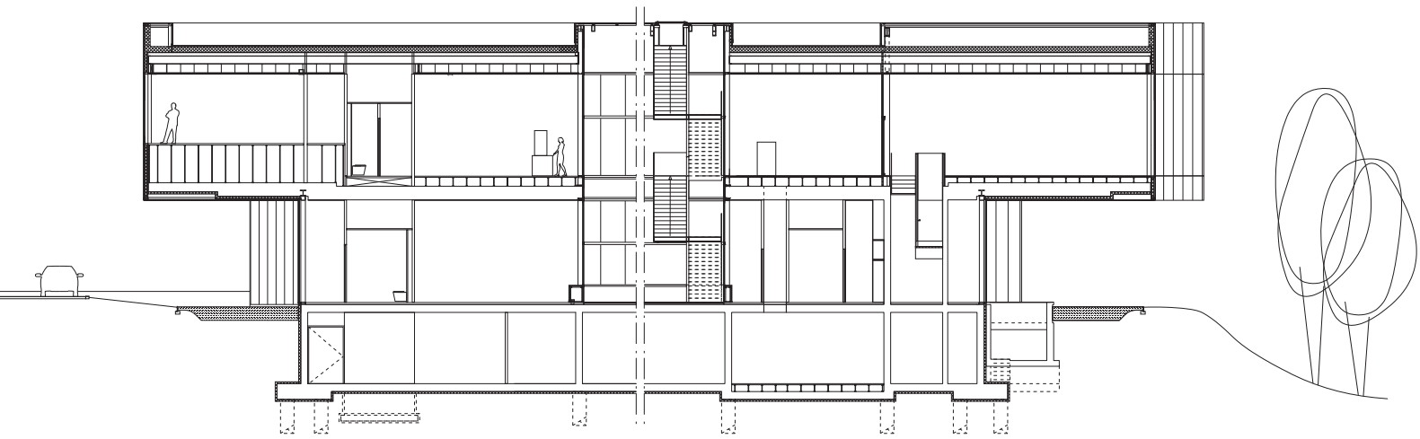
SECTION AA
