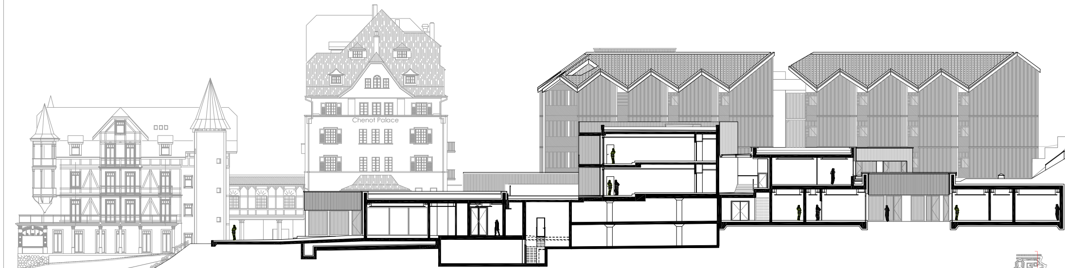
LONG SECTION
