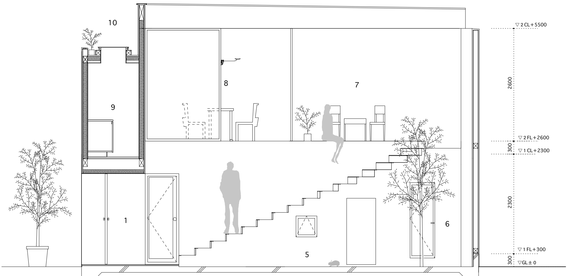
SECTION S= 1/50
