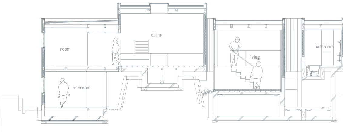
SECTION 1:150
