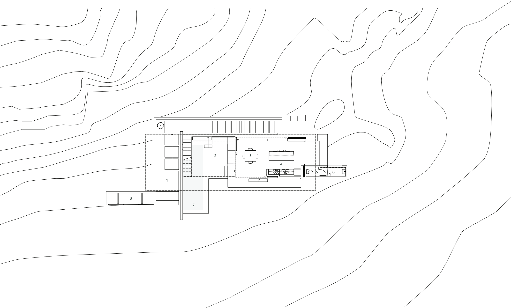
Main Floor Plan 1-entry 2-exterior living space 3-dining 4-kitchen 5-toilet room 6-outdoor shower 7-pool 8-mechanical
