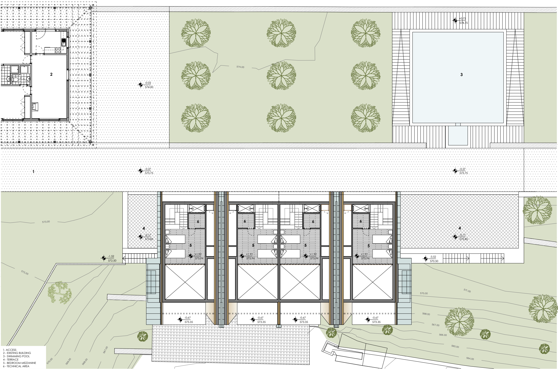
1F FLOOR PLAN
