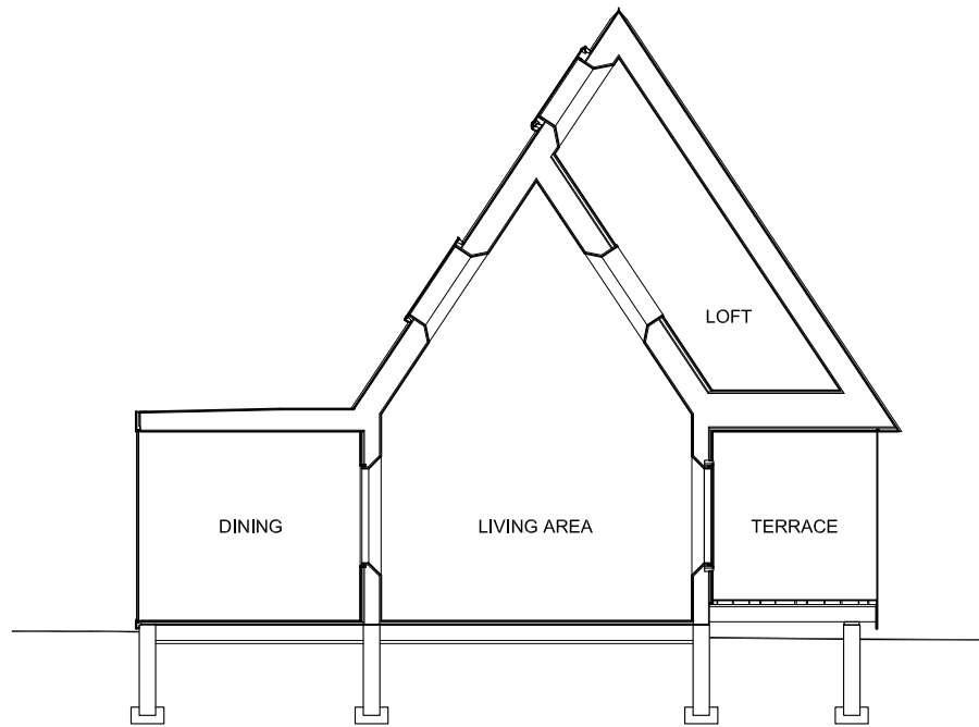
SECTION 1:100
