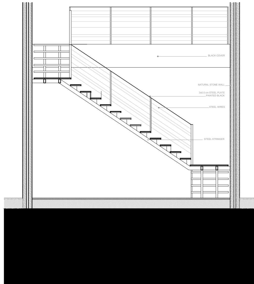
STAIR DETAIL
