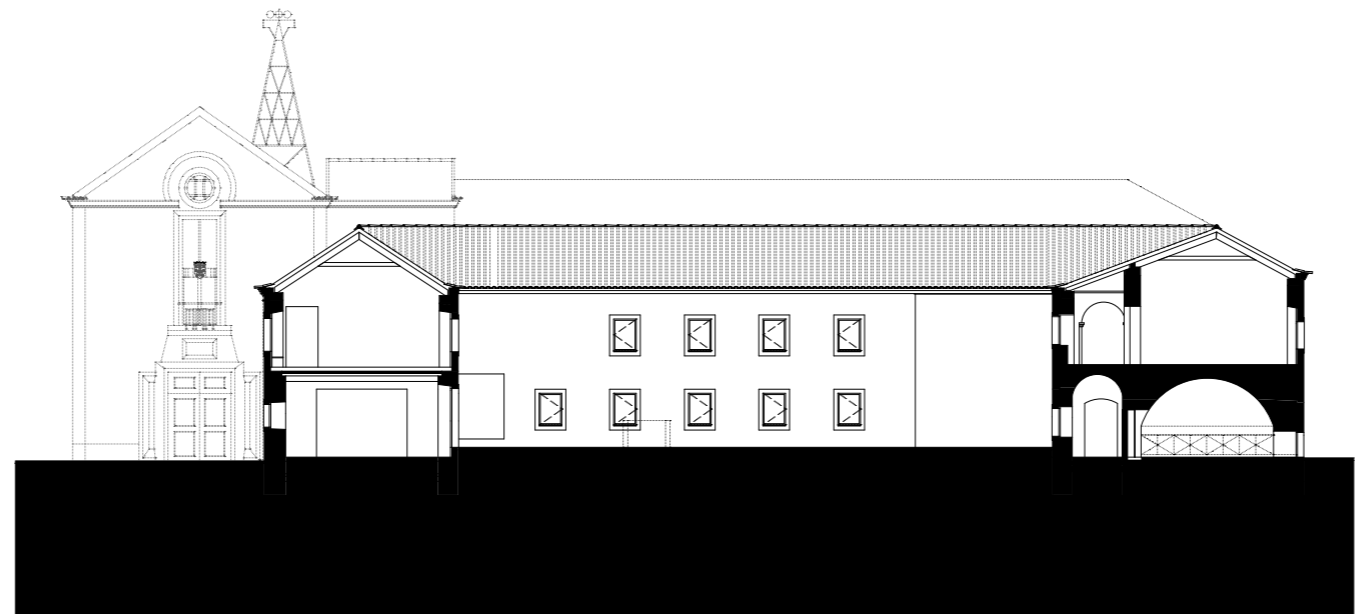
corte 4-4'. section 4-4'
