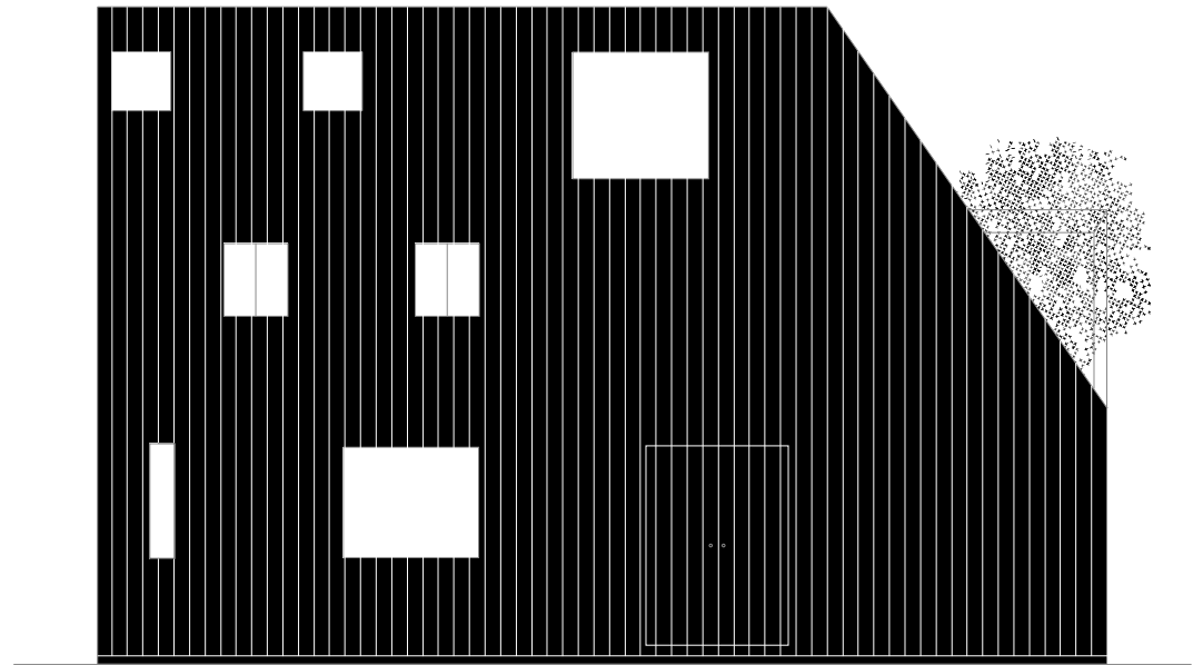
east elevation 1:100
