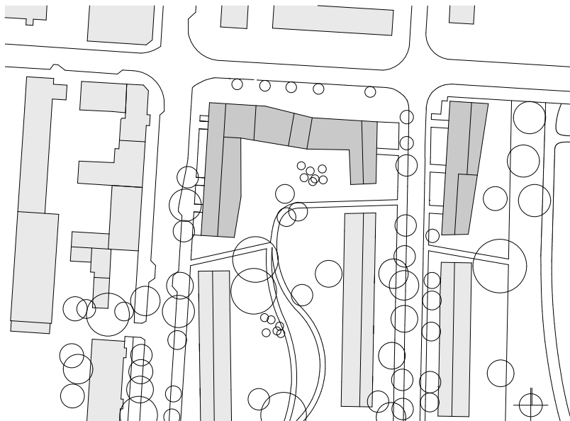
Weltquartier Wilhelmsburg Lageplan M 1_2000
