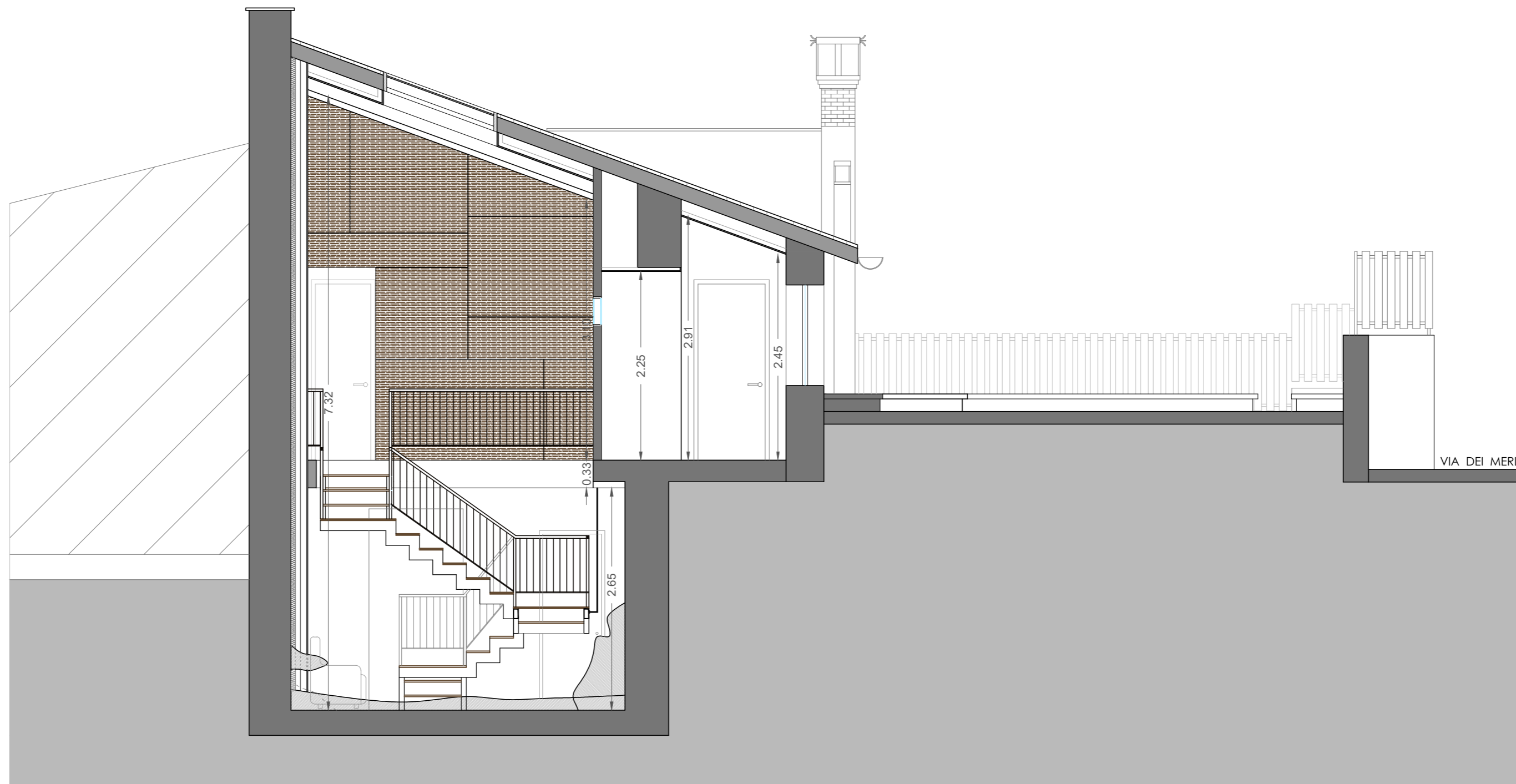
SECTION
