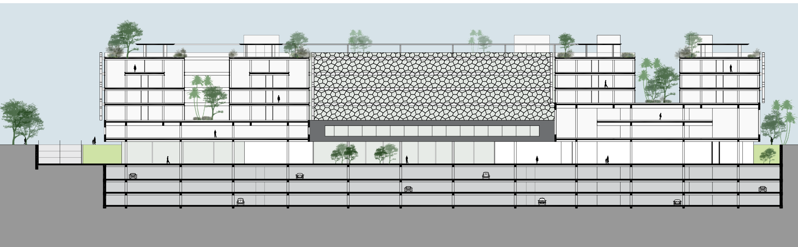
CORTE C SECTION C 0 5 10 50
