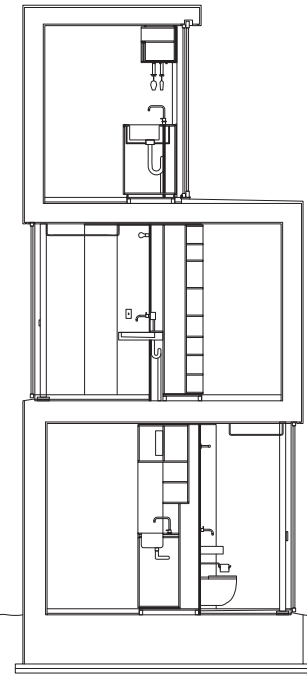
cross section
