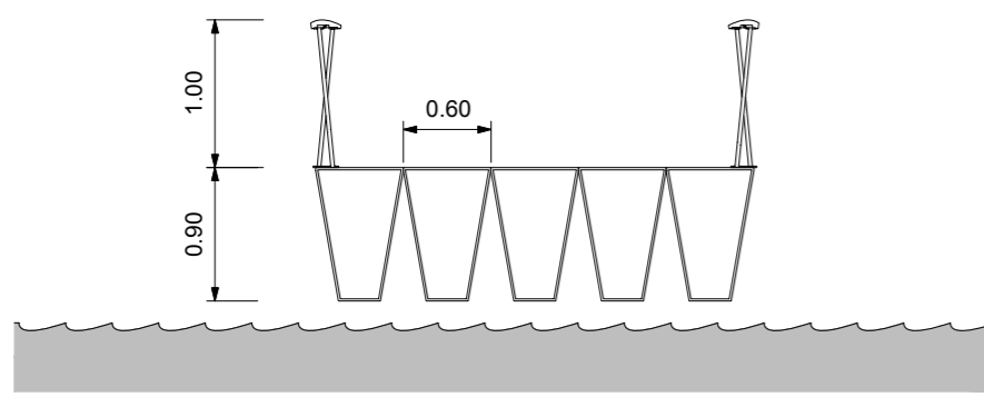
cross section 1:50
