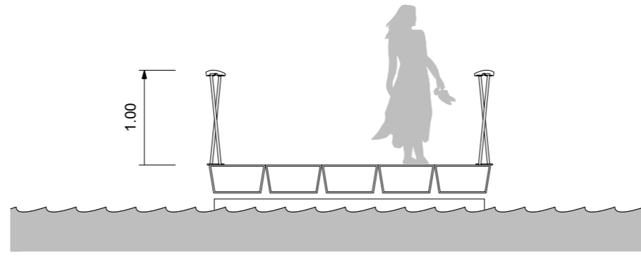
cross section 1:50
