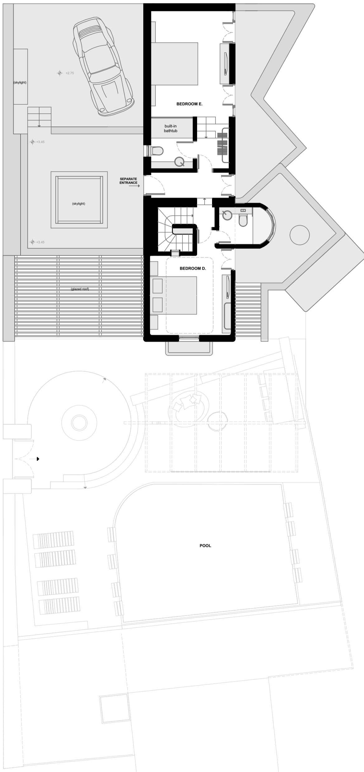
House in Chora Upper Level Scale 1/100
