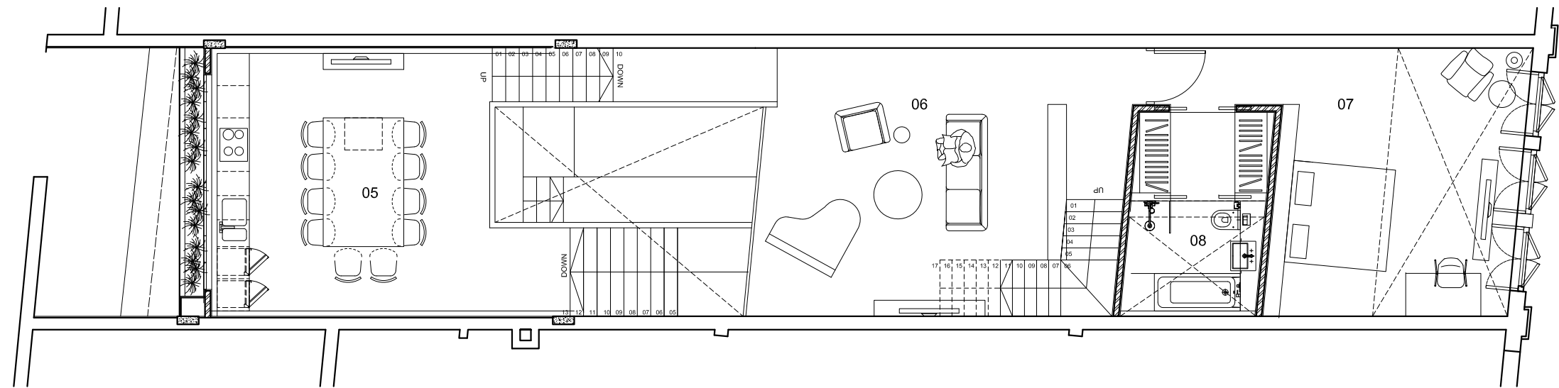
2ND STOREY PLAN
