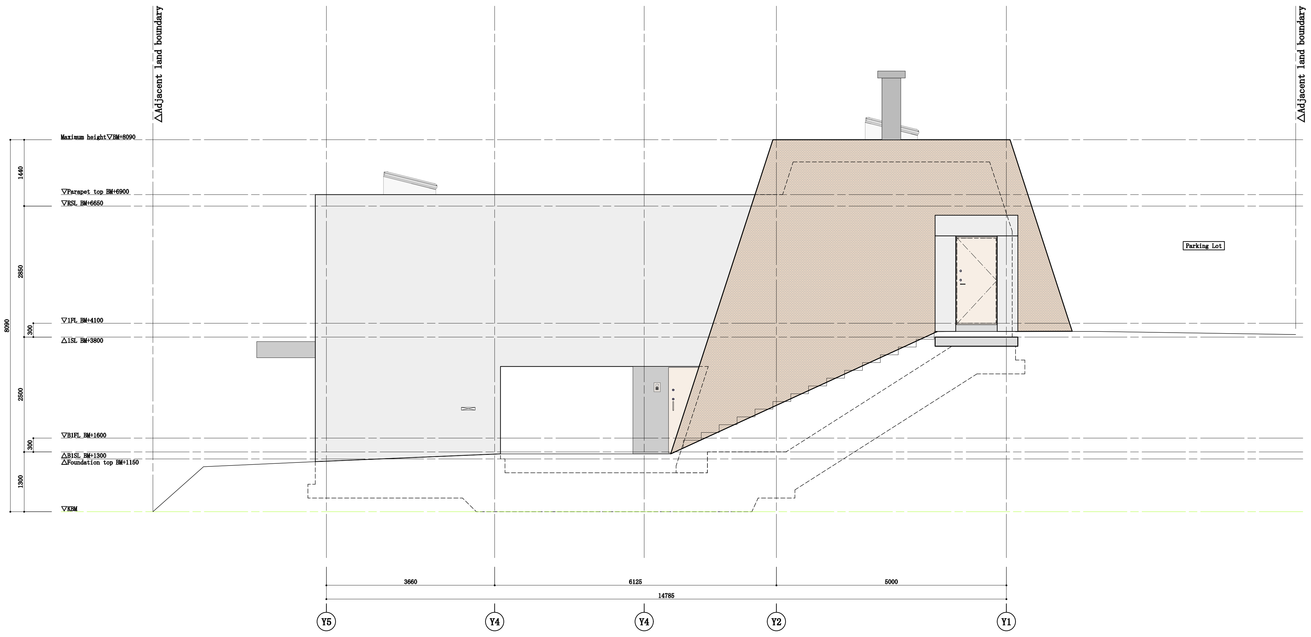
West elevation 1:50
