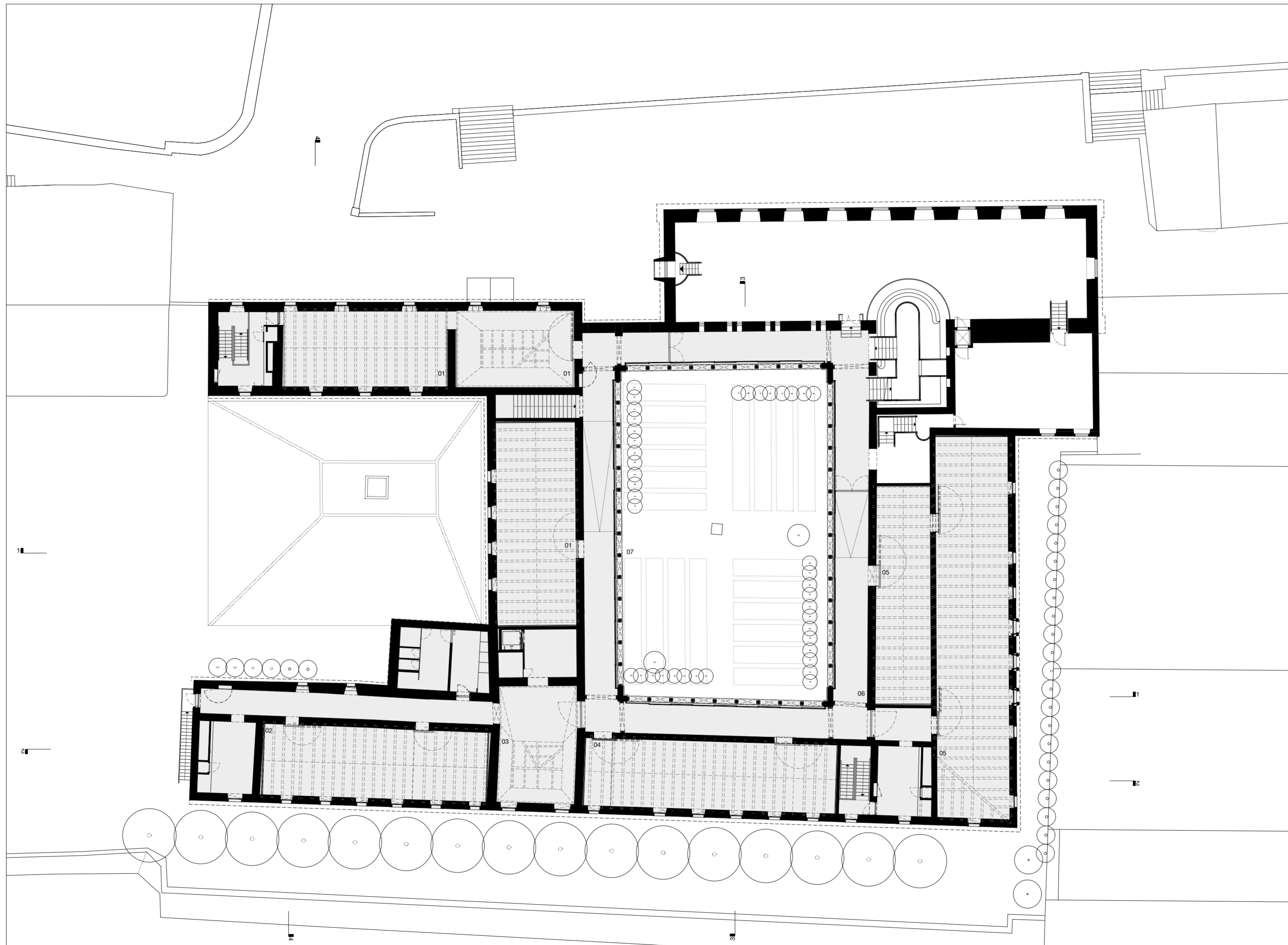
Planta piso 1 — First floor plan
