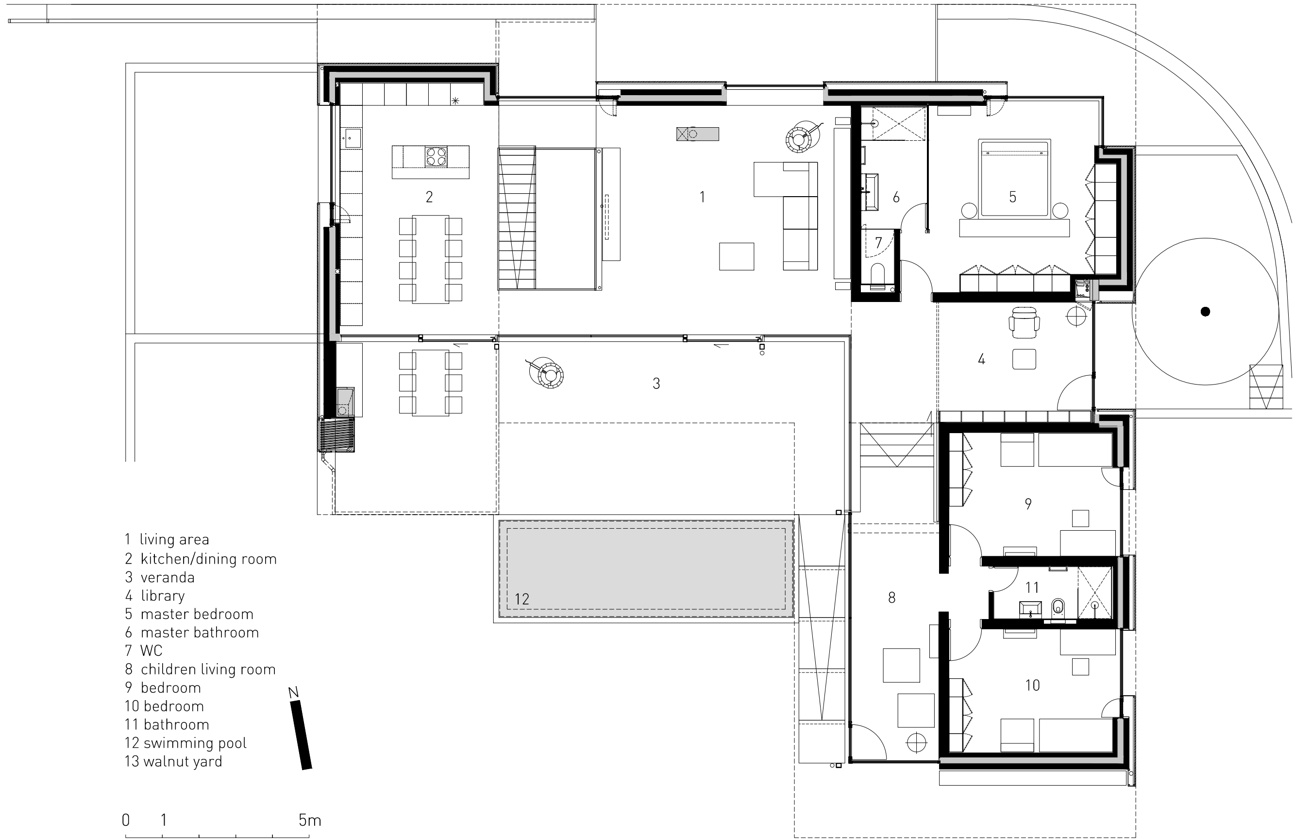
floor plan level 2
