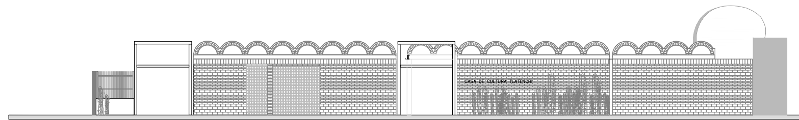
WEST ELEVATION
