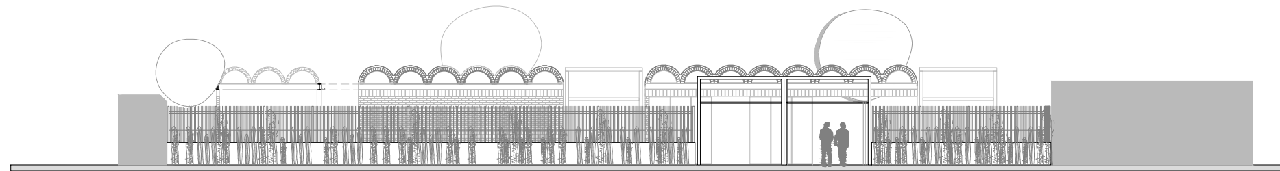
EAST ELEVATION
