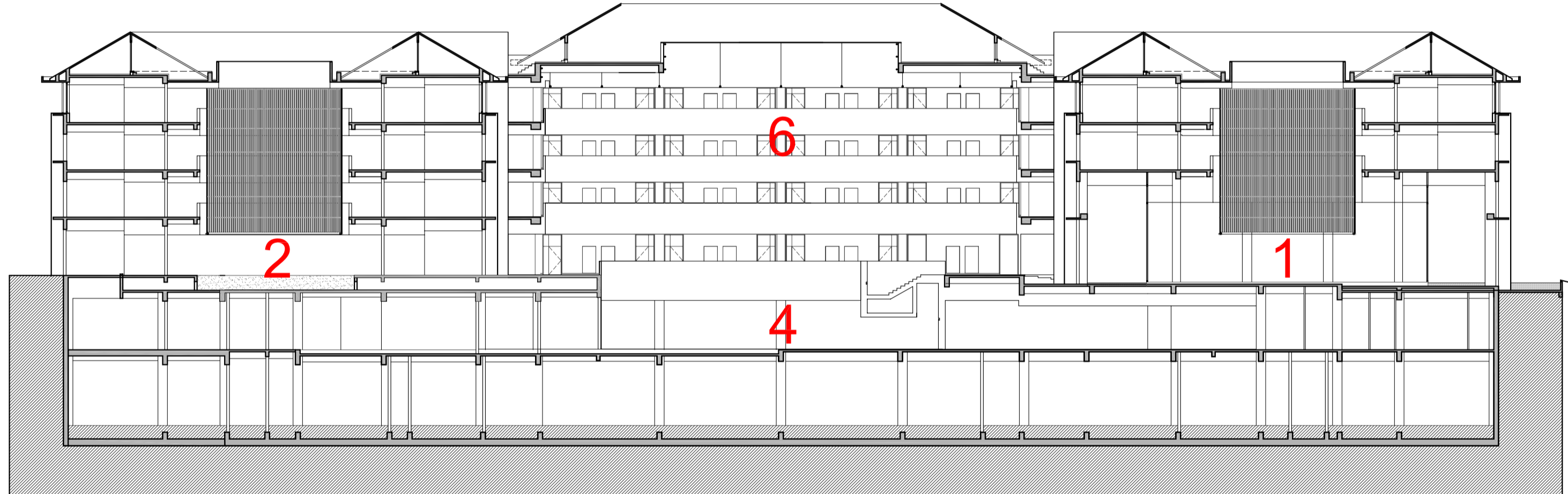
SECTION B-B
