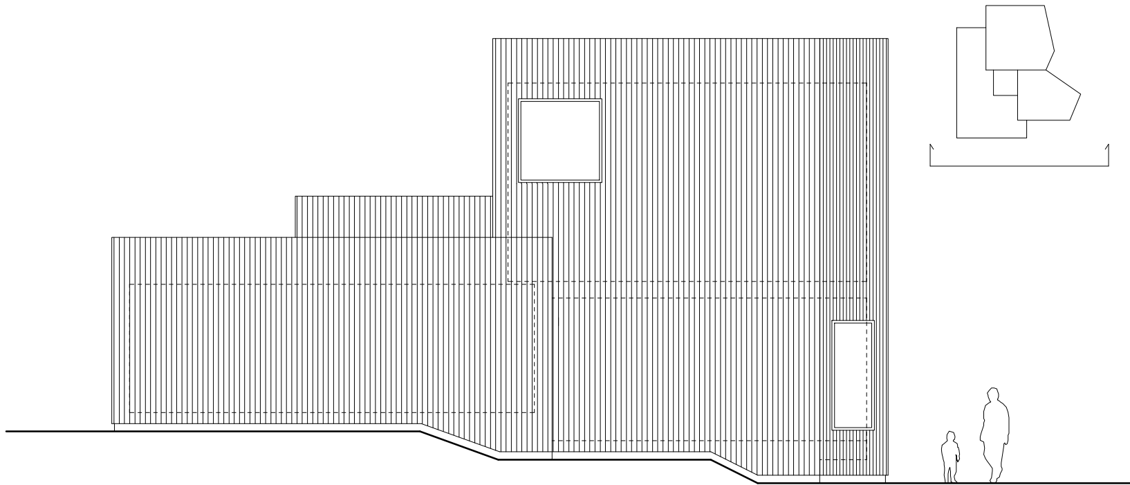
Facade/north 1 : 50
