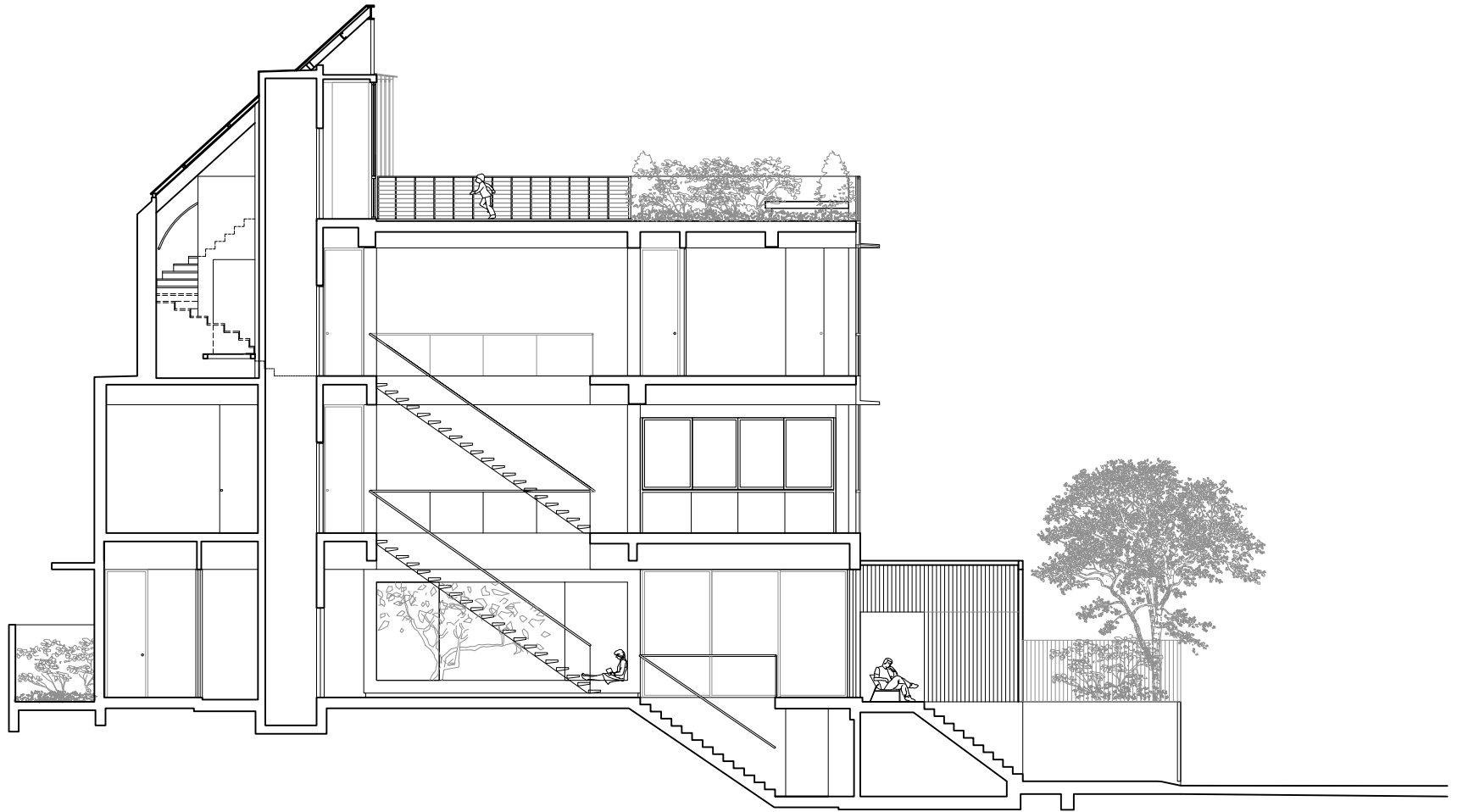
SECTION ACROSS STAIRCASE
