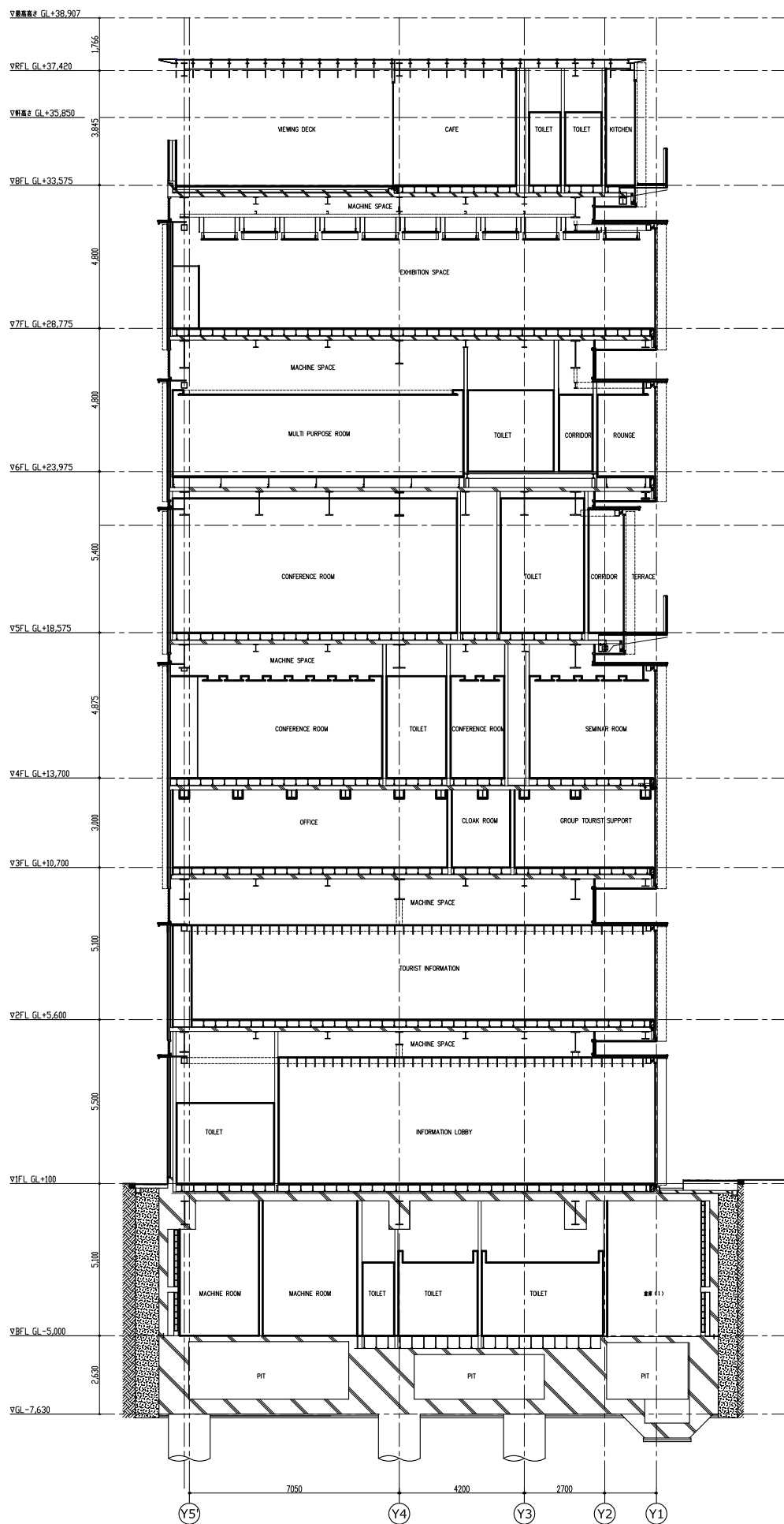
AA' SECTION
