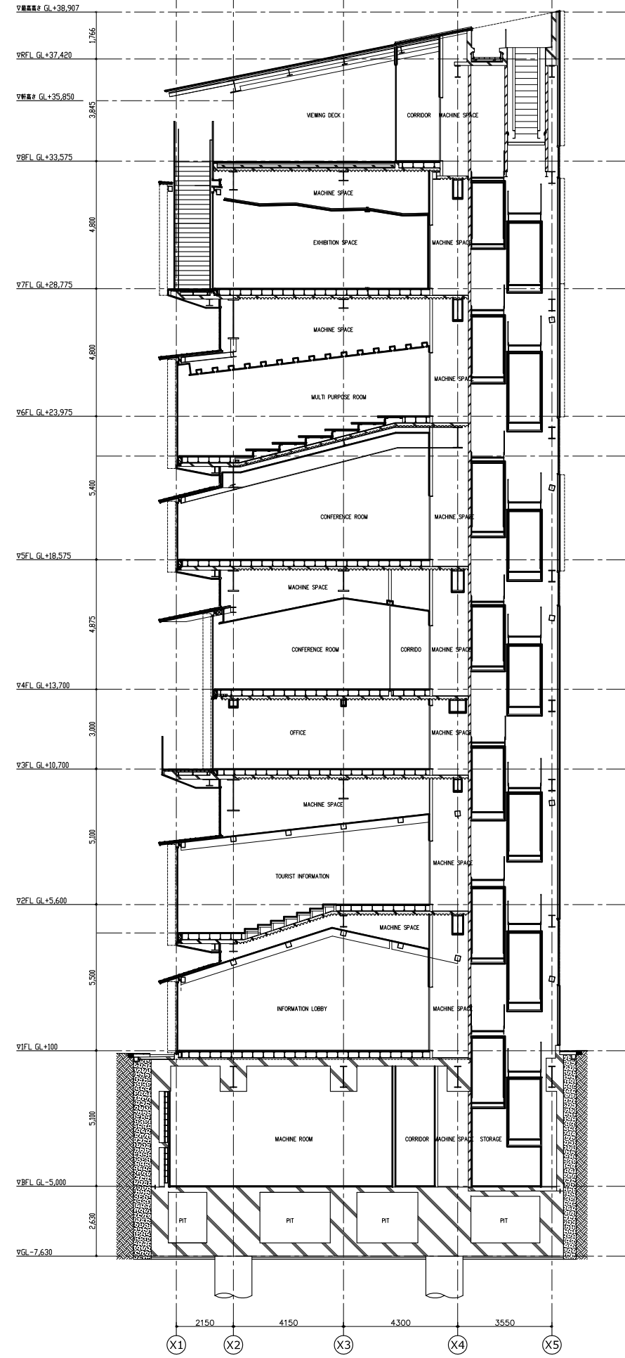
BB' SECTION
