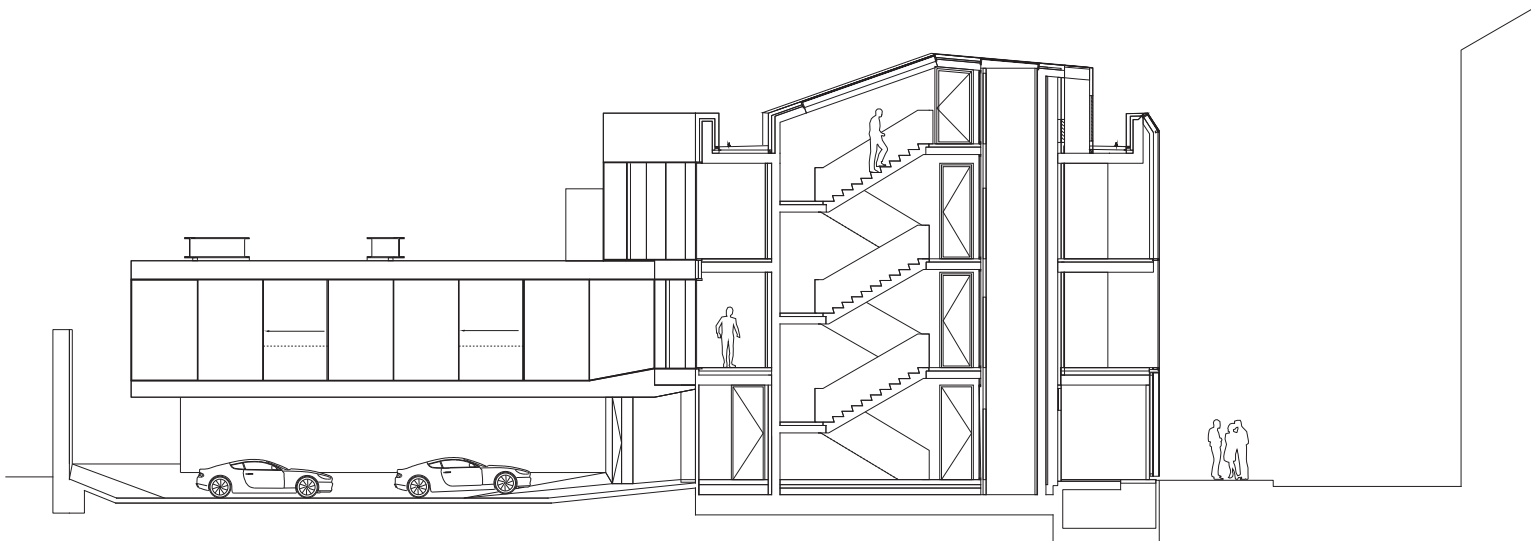
SECTION BB
