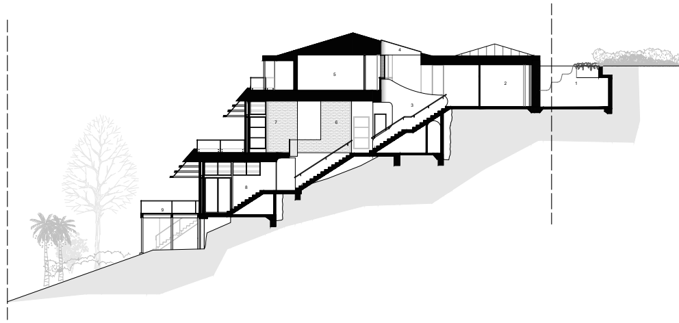
SECTION D-b 0 2 5 10 1. living bedroom 2. porch 3. stairs 4. wall 5. window 6. external staircase 7. external staircase 8. internal staircase 9. external staircase
