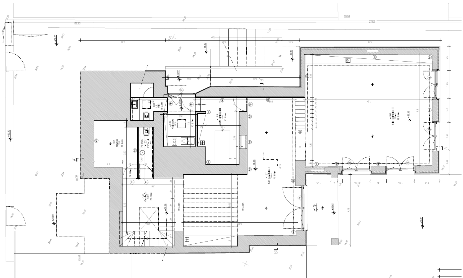
PLAN. 00 (RD - 1) ES. 1/50
