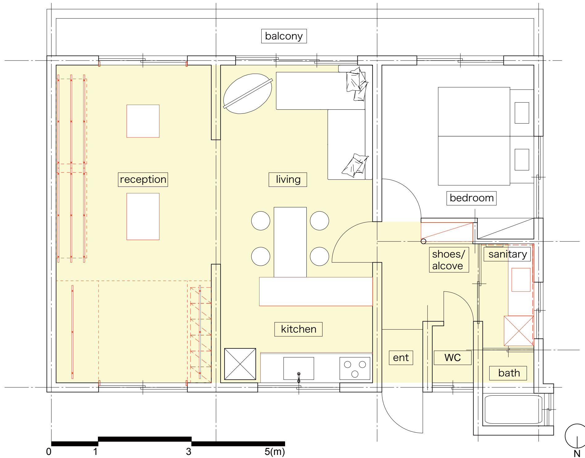
after renovation plan S=1/50
