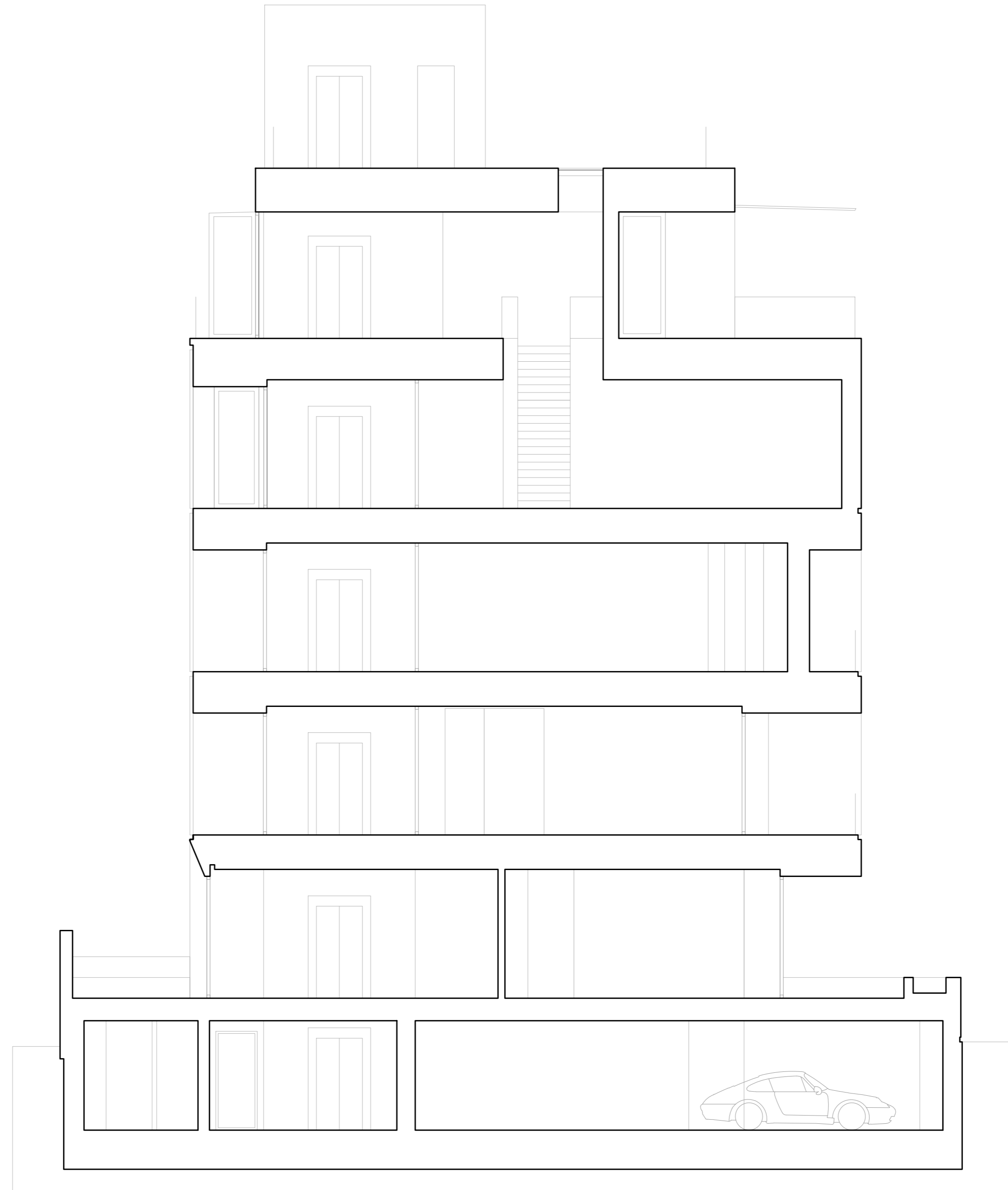
CROSS-SECTION
