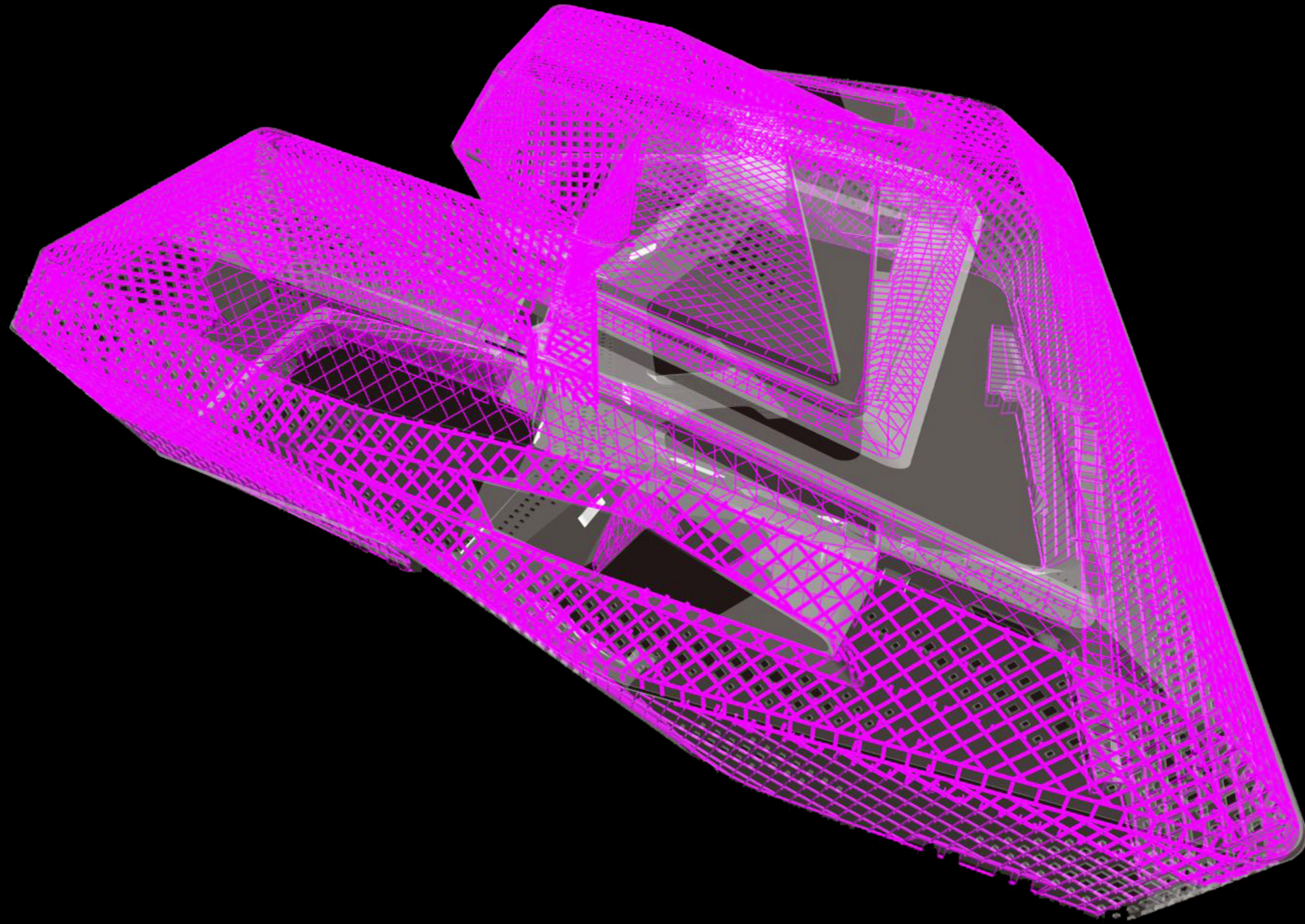
Nanjing International Youth Cultural Centre BIM MODEL - Secondary Steel Structure
