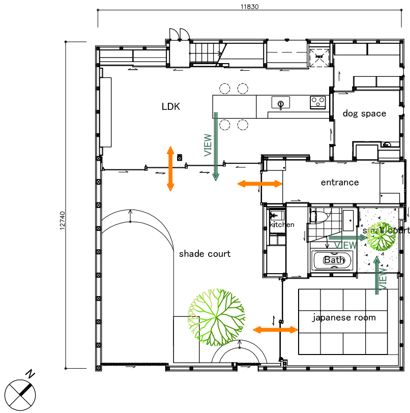
1st floor S=1/150
