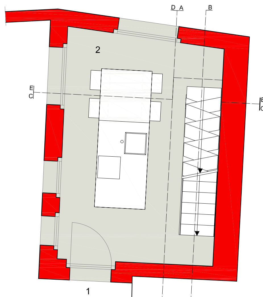
PIANO TERRA
