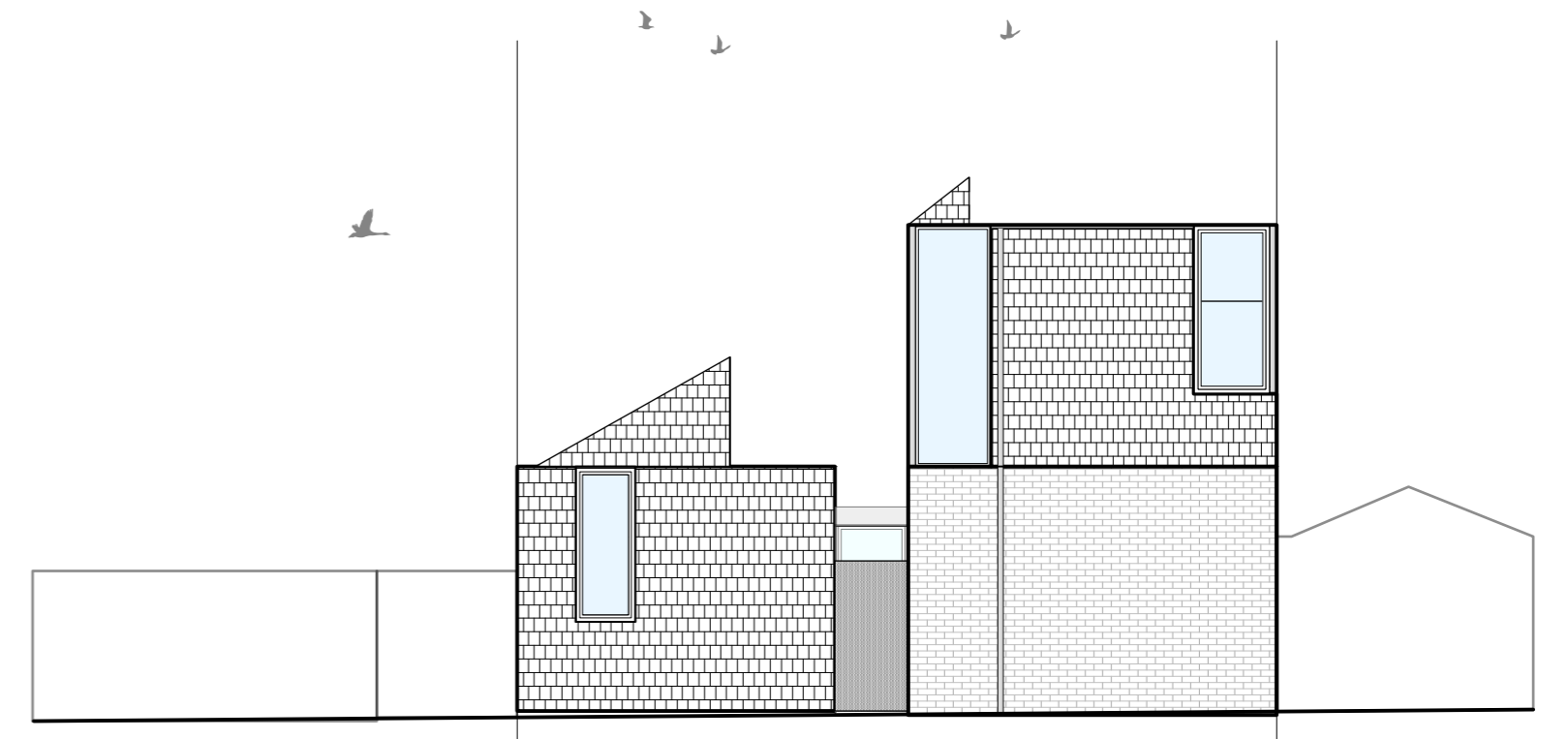
Elevation South
