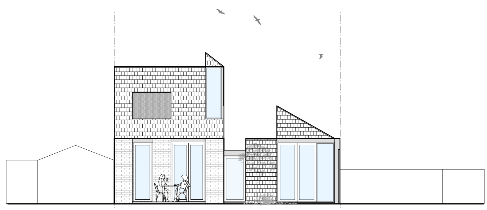
Elevation North
