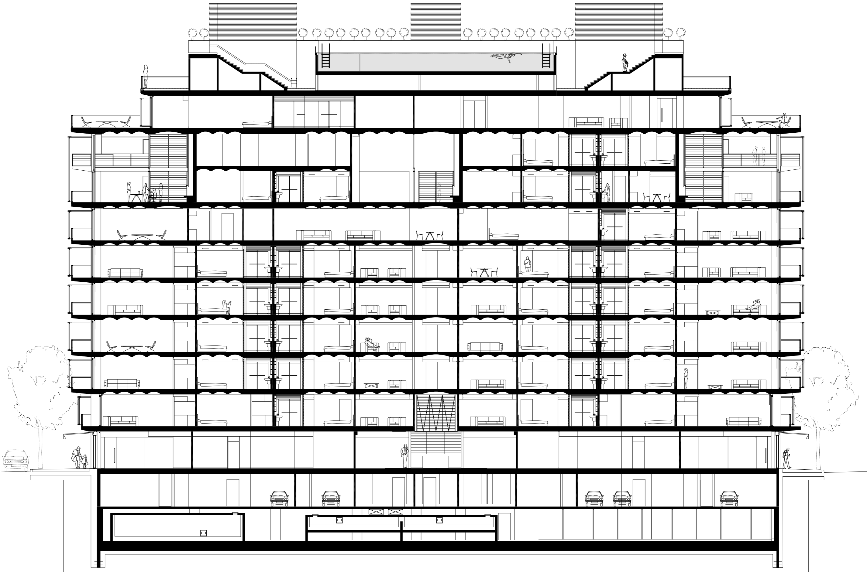
The Aleph: Long Section
