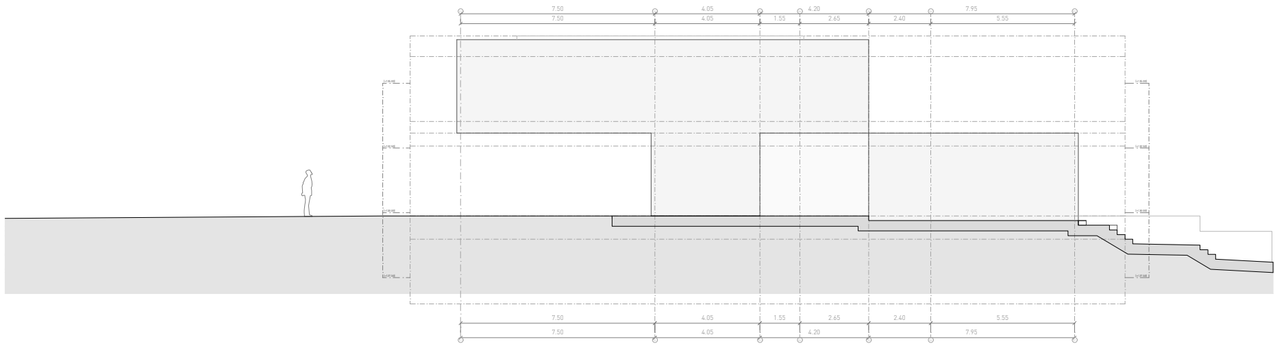
HOUSE IN THE LAKE | CASA EN EL LAGO SOUTHEAST AND NORTHWEST ELEVATIONS | ALZADOS NOROESTE Y SURESTE
