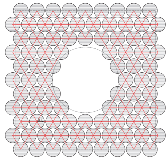
Regular Hexagonal Matrix R1 = 925mm (4-seater Pods)
