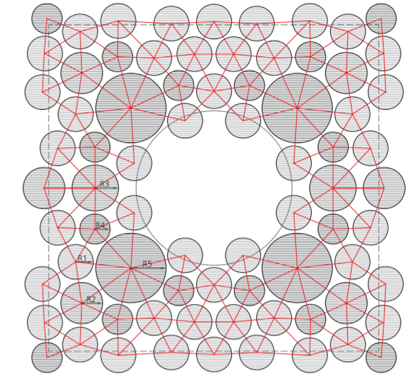
4, 6, 8 & 12-seater Pods R1 = 925mm (4-seater Pods) R2 = 1100mm (6-seater Pods) R3 = 1225mm (8-seater Pods) R4 = 825mm (Access Pods) R5 = 1850mm (12-seater Pods)
