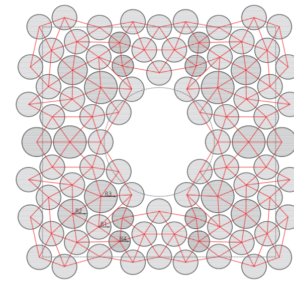
Access Pods R1 = 925mm (4-seater Pods) R2 = 1100mm (6-seater Pods) R3 = 1225mm (8-seater Pods) R4 = 825mm (Access Pods)
