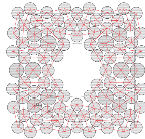
4, 6 & 8-seater Pods R1 = 925mm (4-seater Pods) R2 = 1100mm (6-seater Pods) R3 = 1225mm (8-seater Pods)
