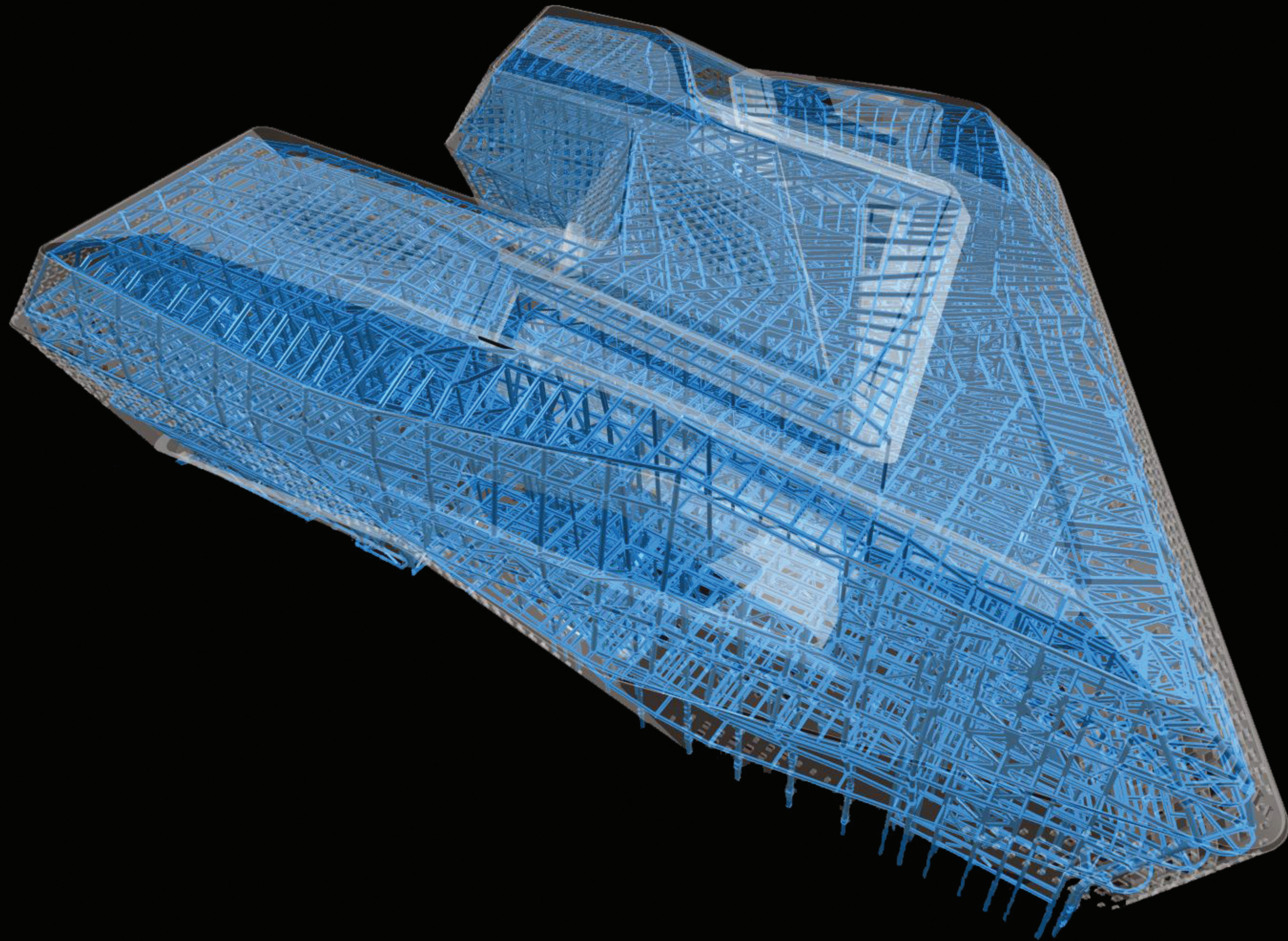
Nanjing International Youth Cultural Centre BIM MODEL - Primary Steel Structure
