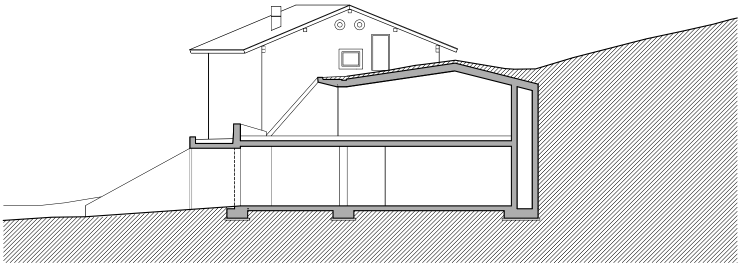
SECTION B-B 1:200
