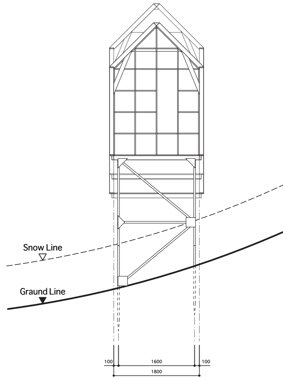
North Elevation S=1/50
