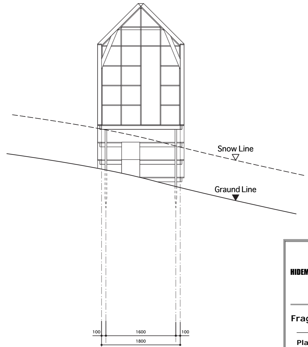
South Elevation S=1/50
