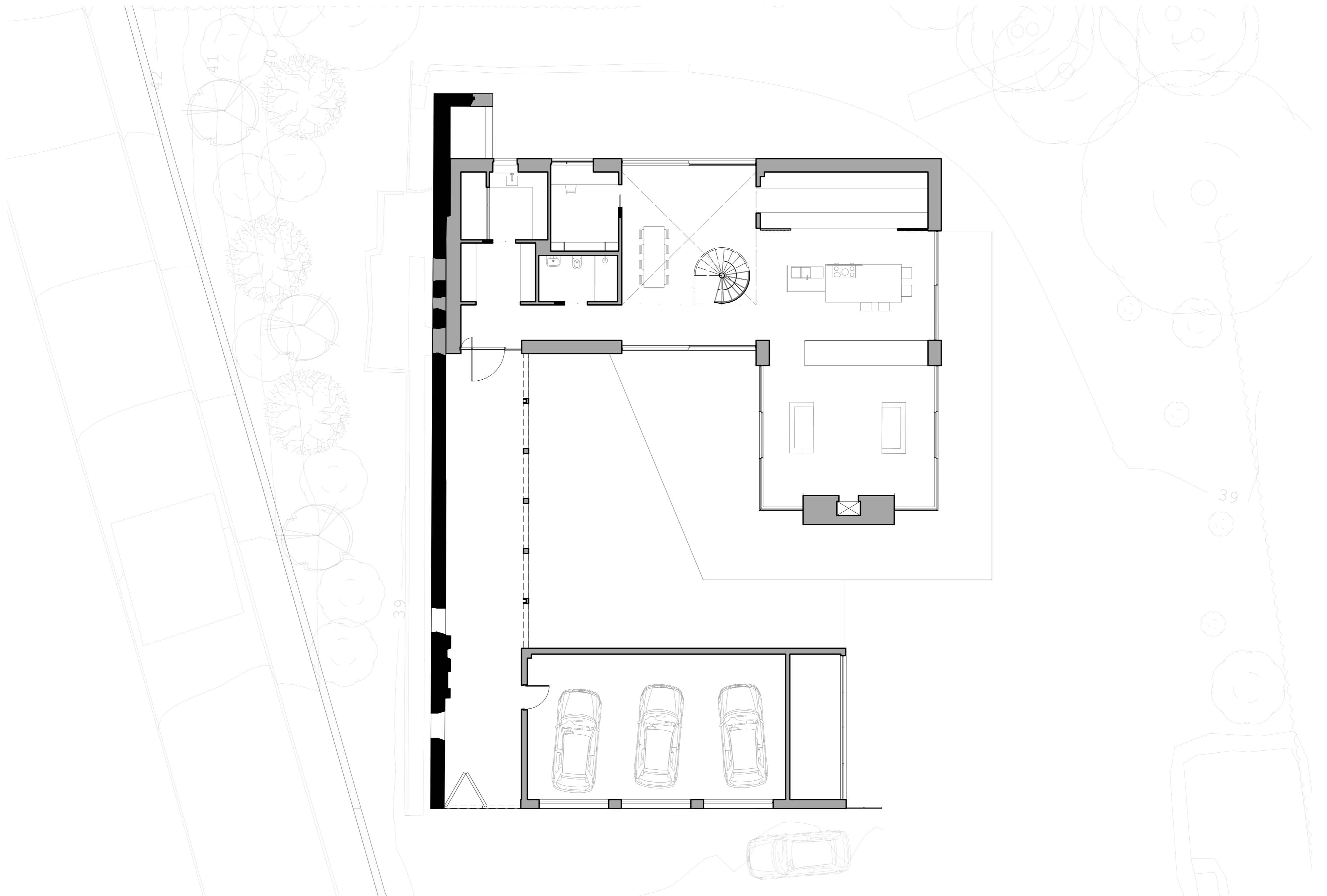
GFPlan
