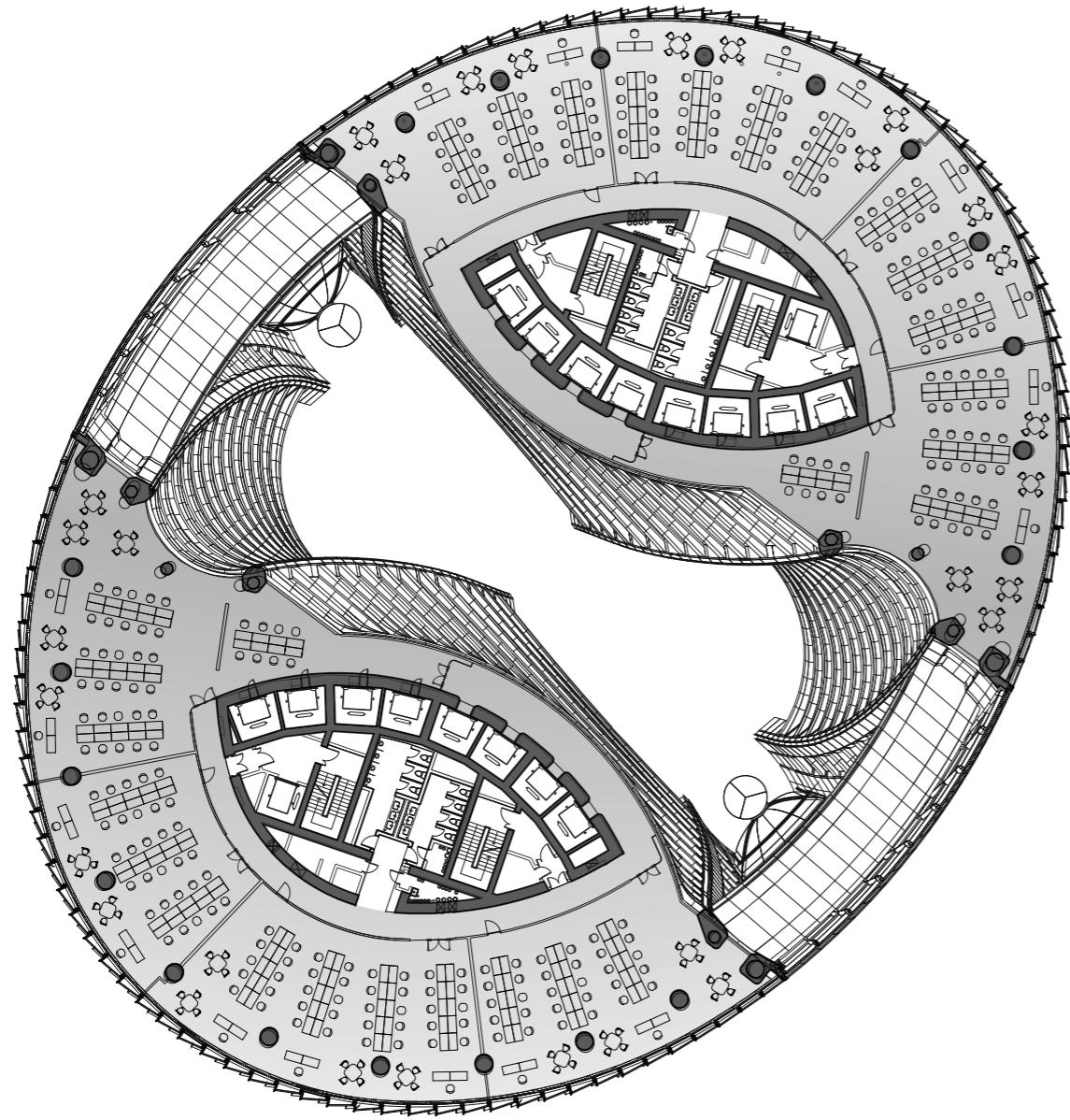
MULTIPLE-UNIT PLAN
