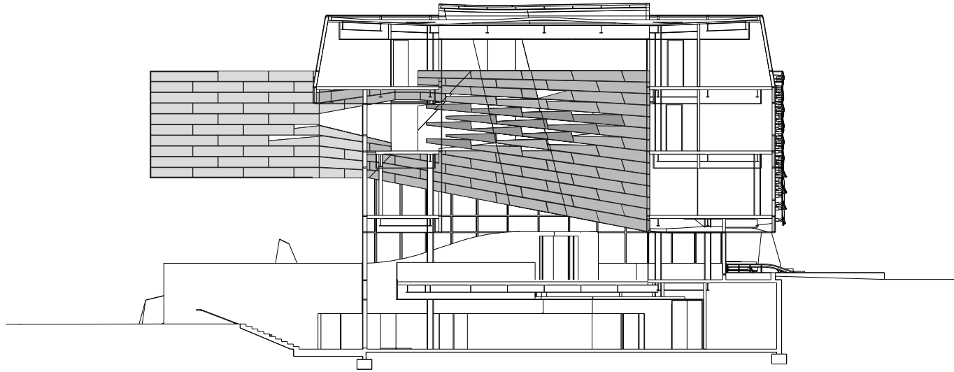
ATRIUM WEST ELEVATION
