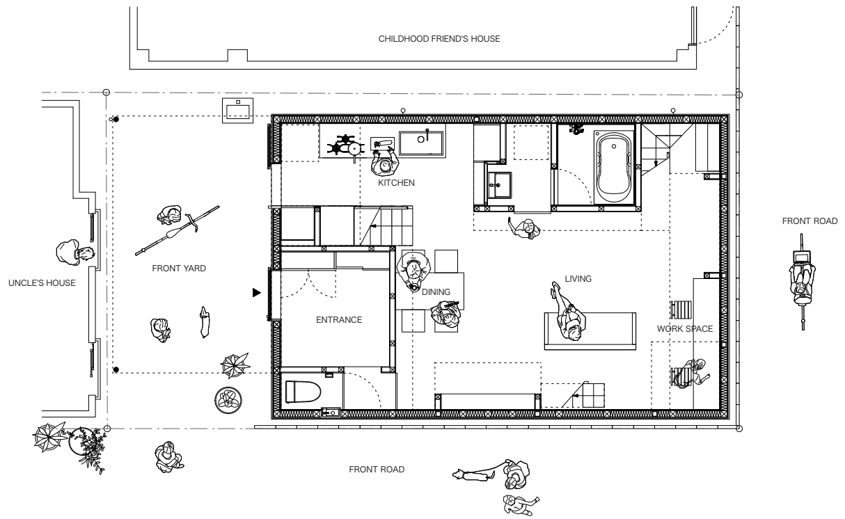
FIRST FLOOR PLAN S=1:100
