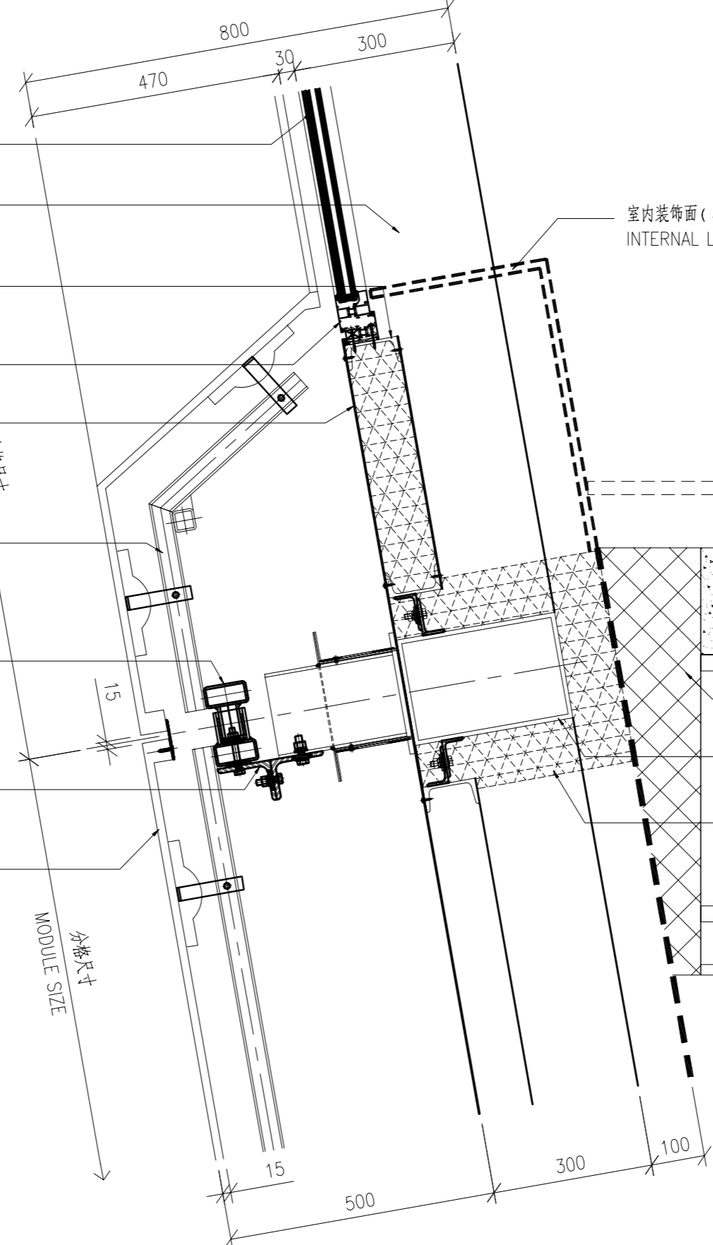
DETAIL - GRC Facade: Interface with windows, Vertical Section. Nanjing International Youth Cultural Centre
